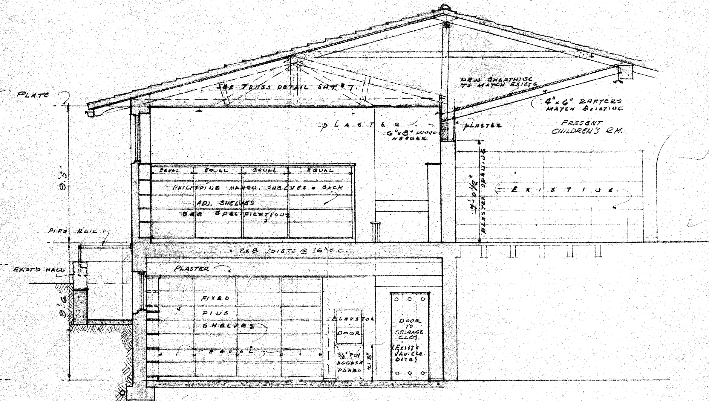
SECTION E-E LOOKING EAST
