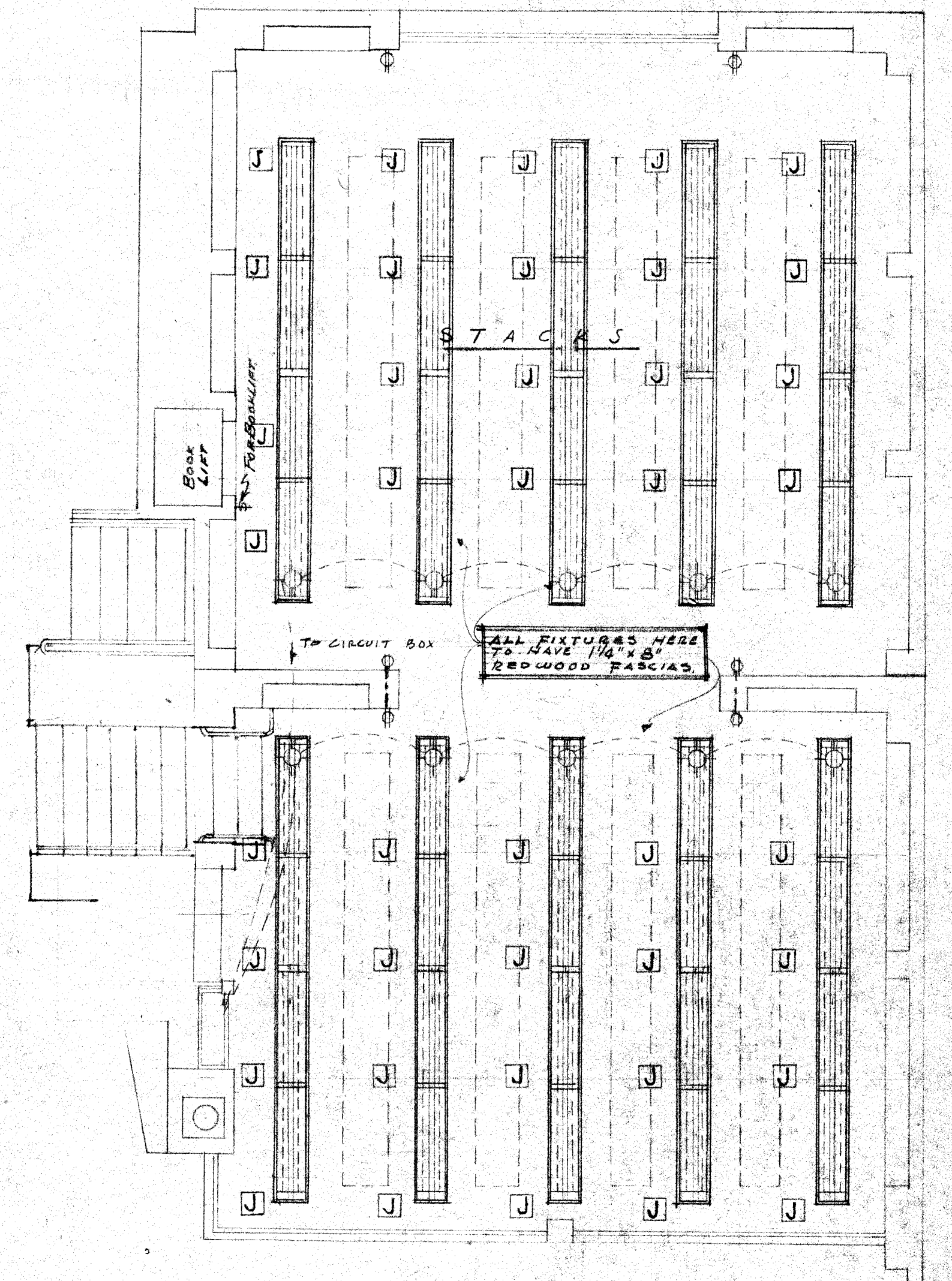
UPPER FLOOR PLAN SCALE 1/4" = 1'-0"
