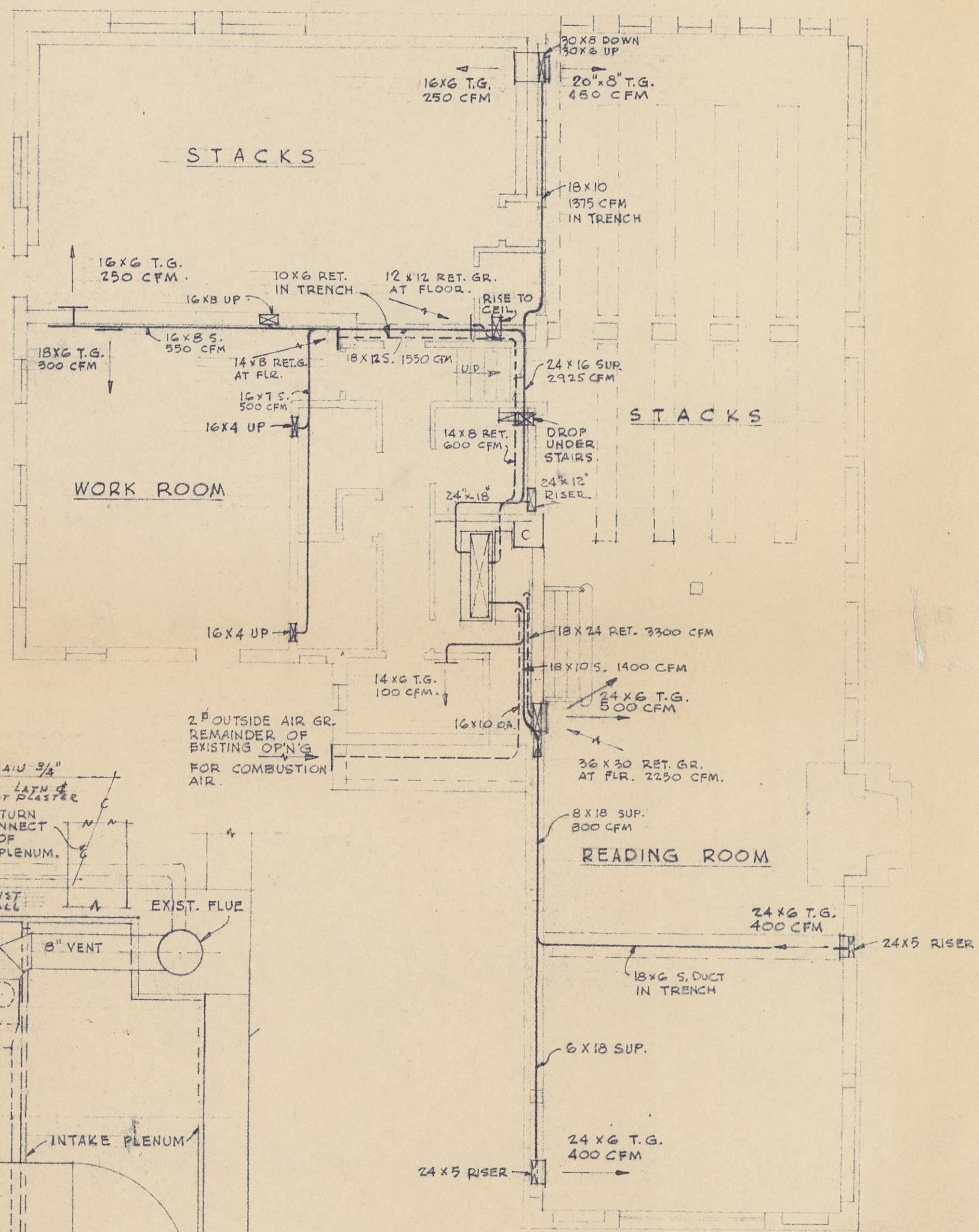
BASEMENT & FIRST FLOOR PLAN SCALE 1/8" = 1'0"
