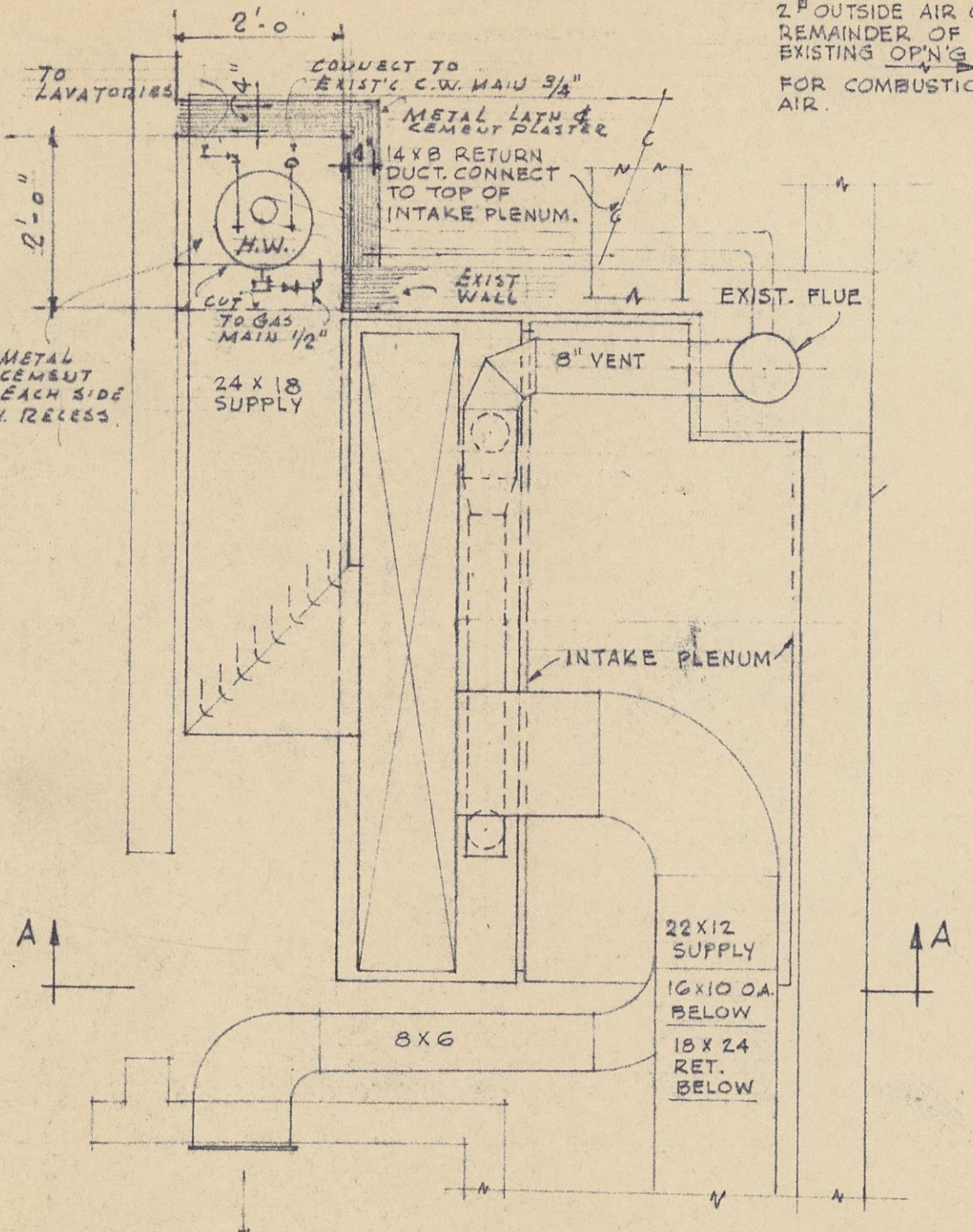
FURNACE ROOM PLAN SCALE 1/2" = 1'0"
