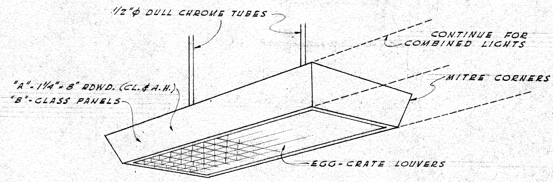
PERSPECTIVE SKETCH OF FIXTURE
