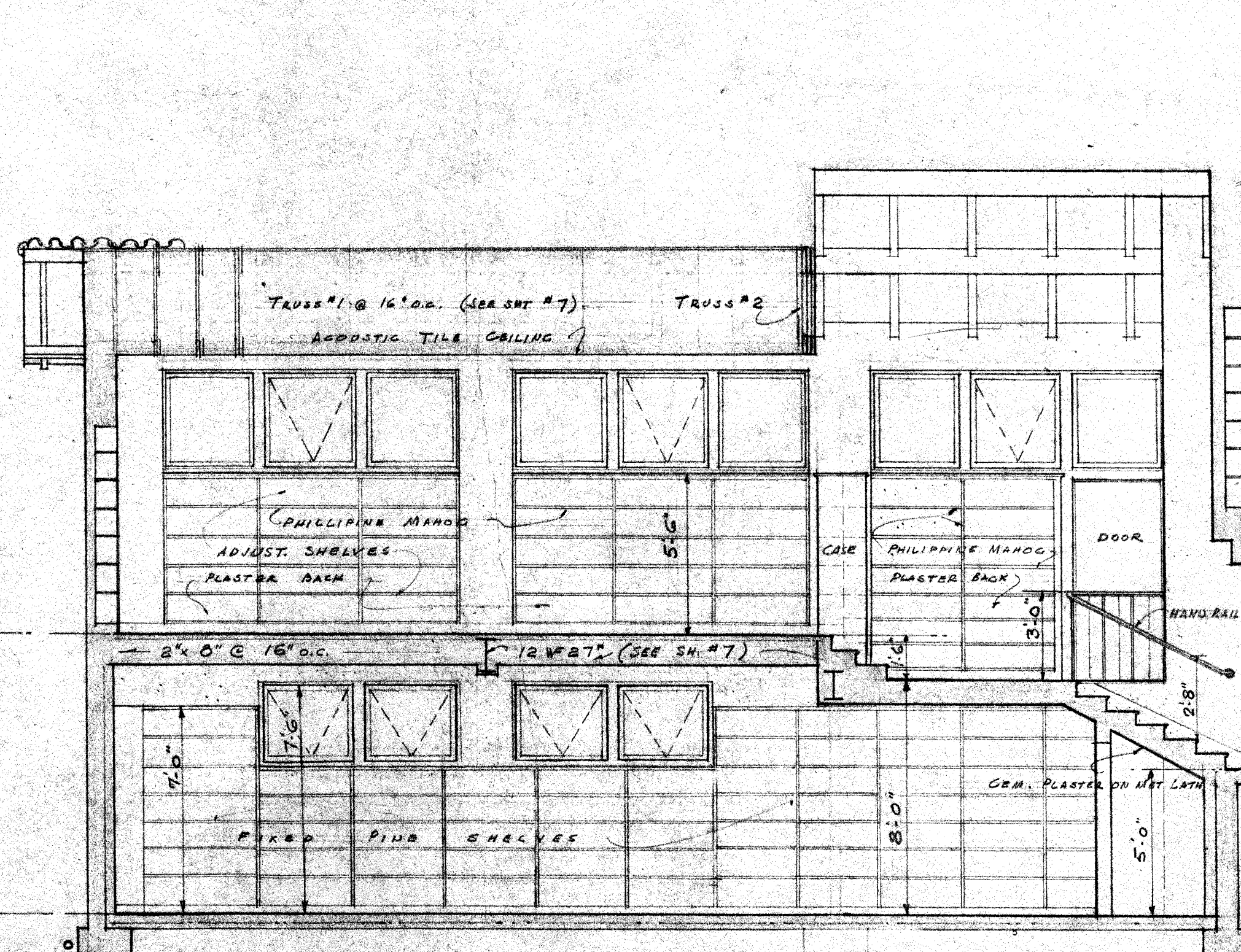
SECTION G-G LOOKING NORTH
