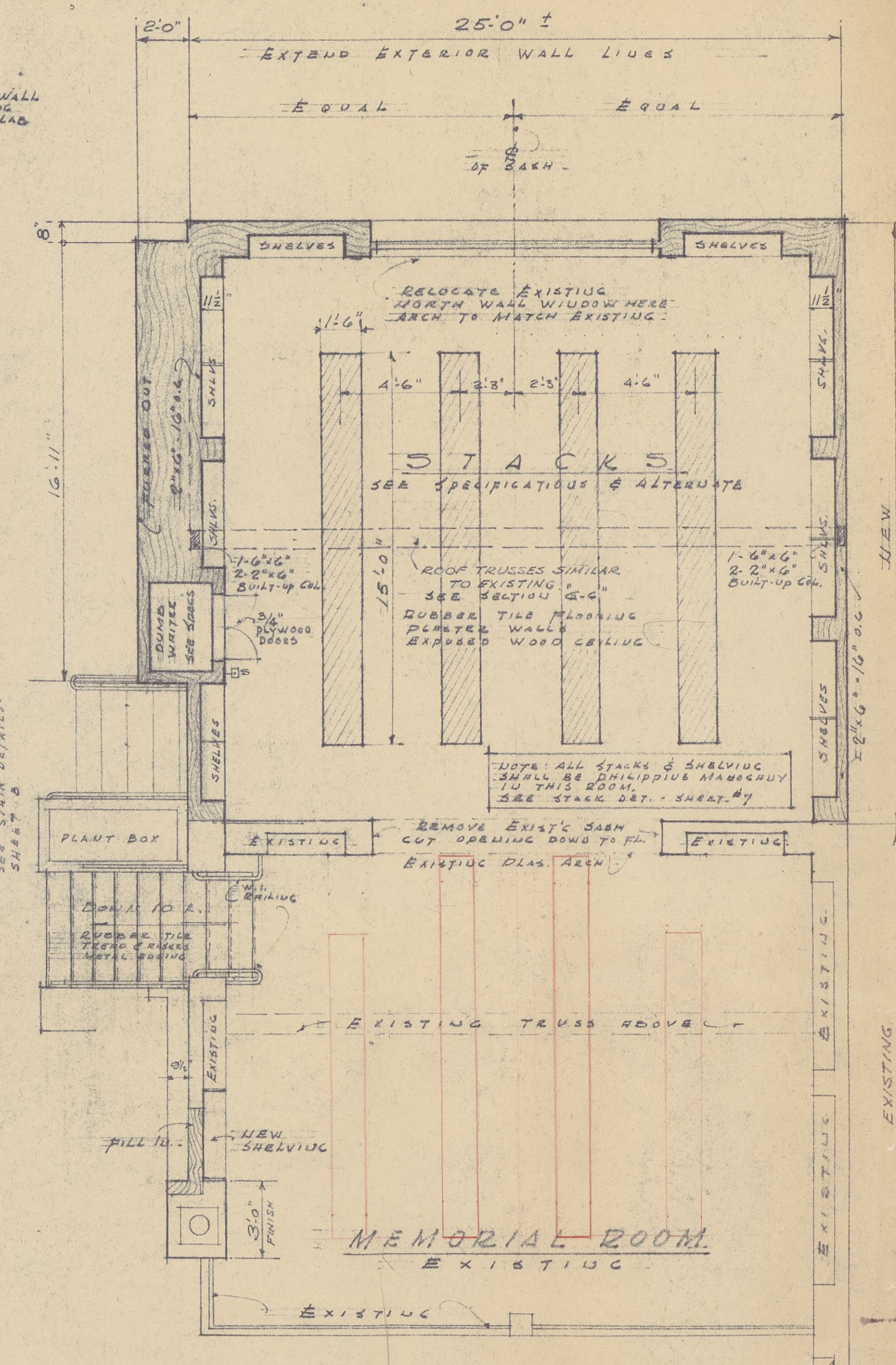
UPPER FLOOR PLAN Scale 1/4" = 1'-0"
