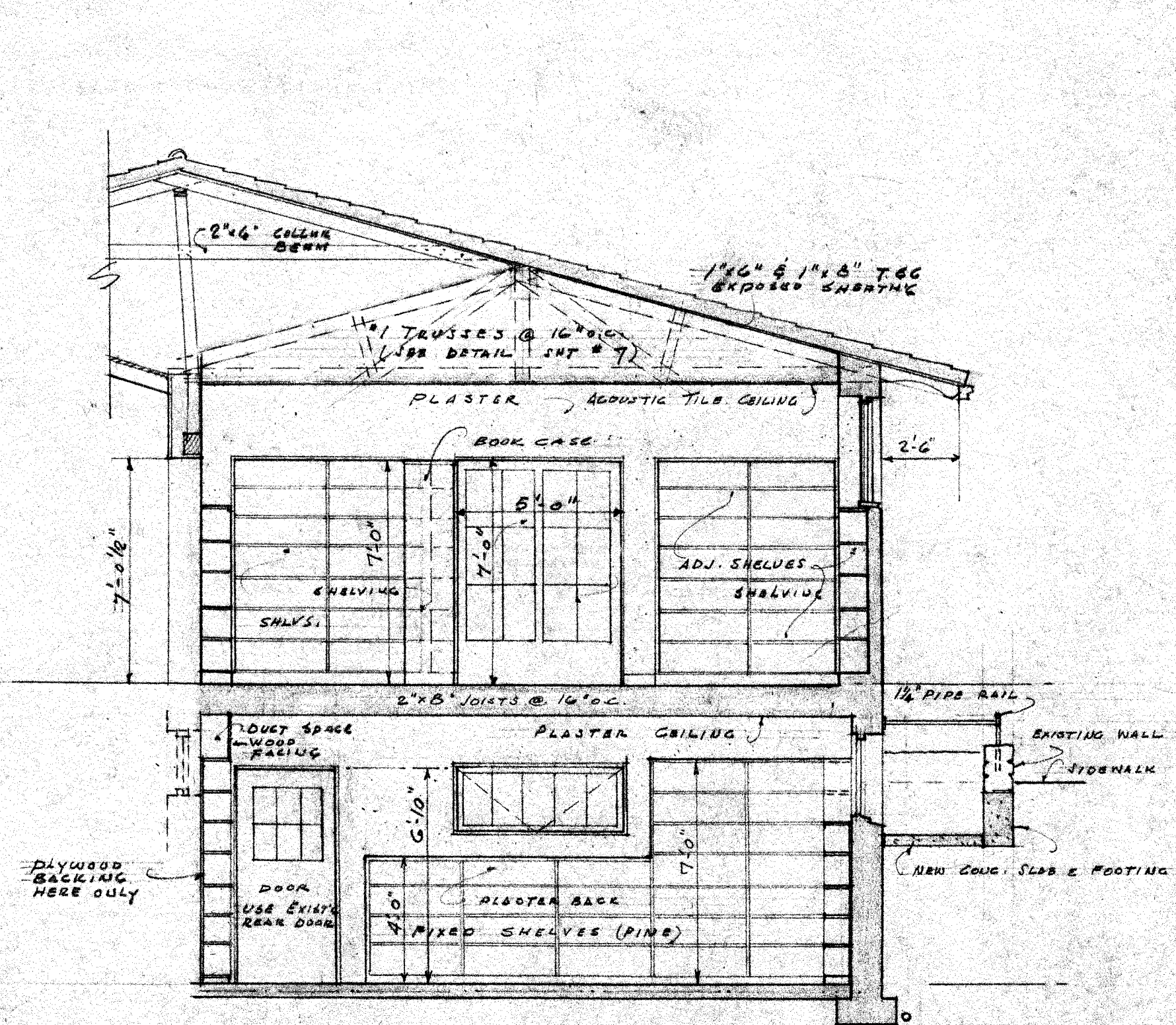
SECTION F-F LOOKING WEST
