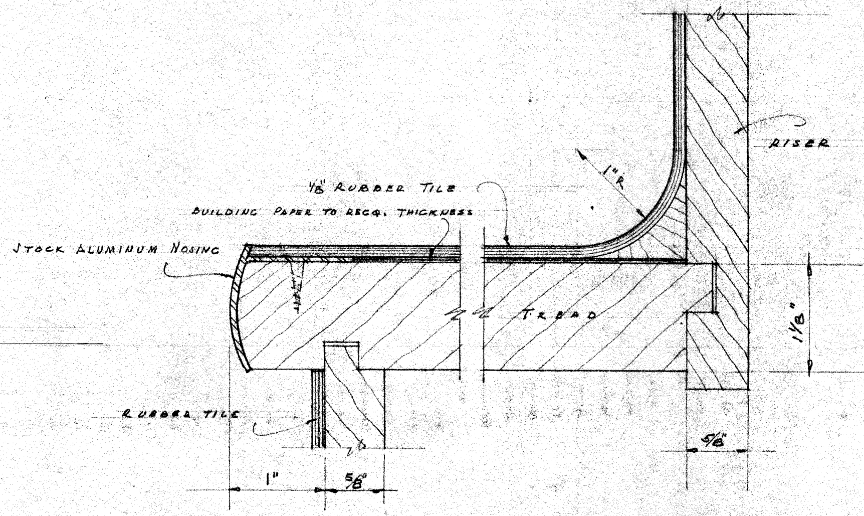
F.S.D. STAIR NOSING & COVE
