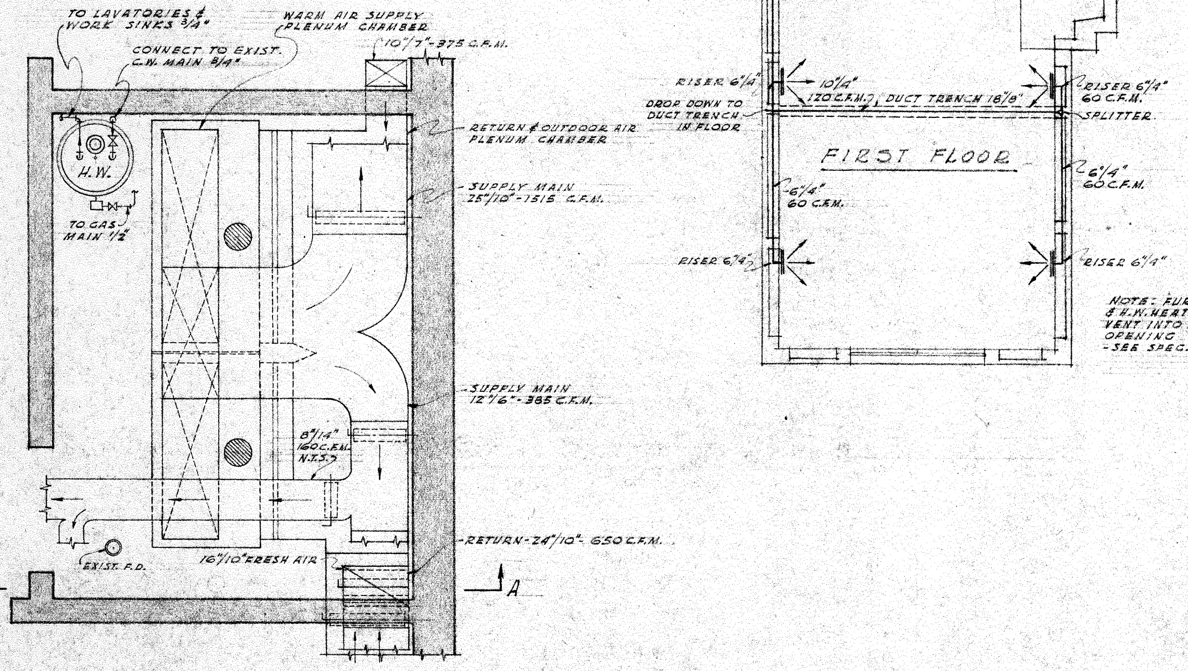
DETAIL OF FURNACE ROOM SCALE: 1/2" = 1'-0"
