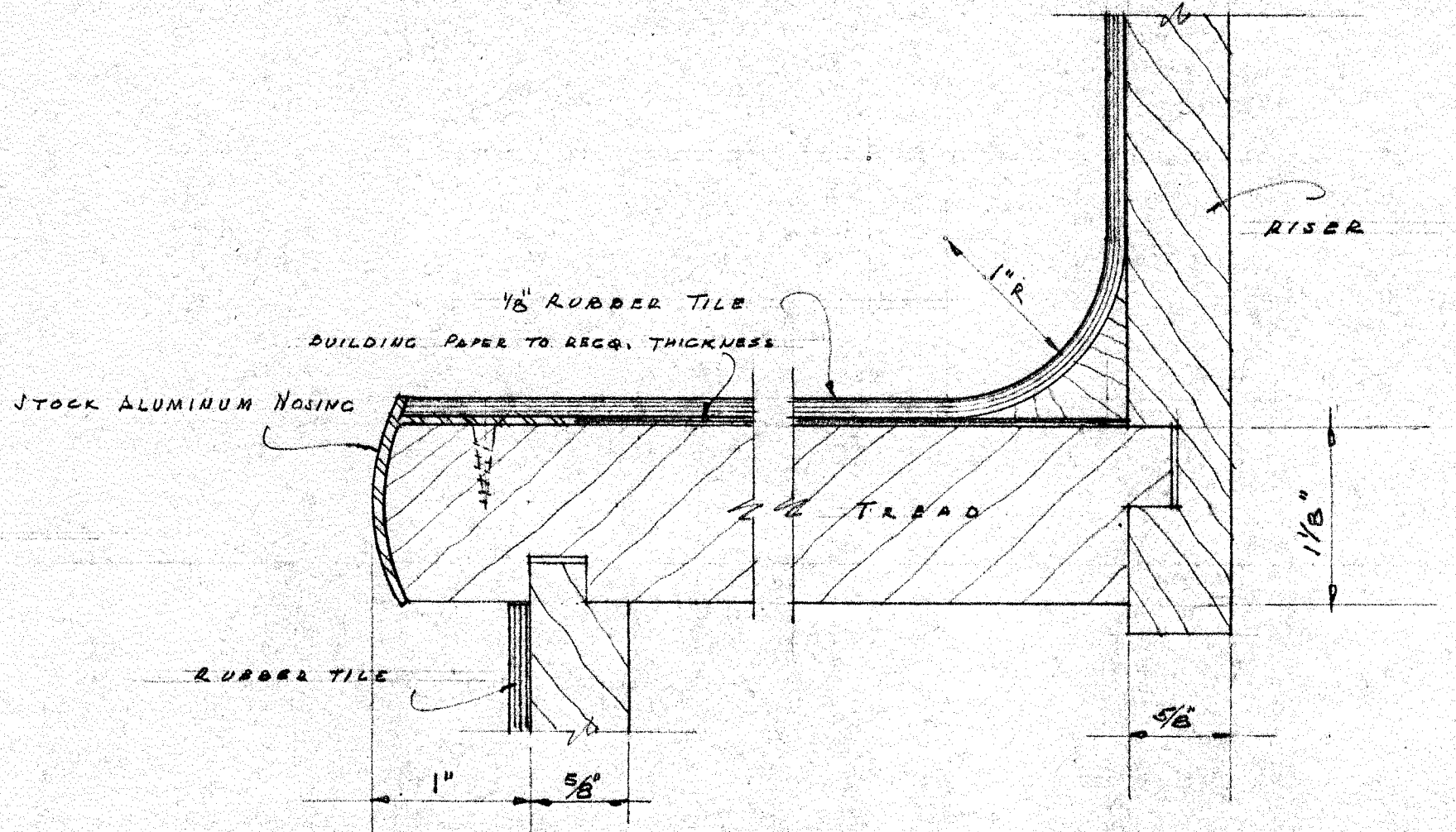
F.S.D. STAIR NOSING & COVE
