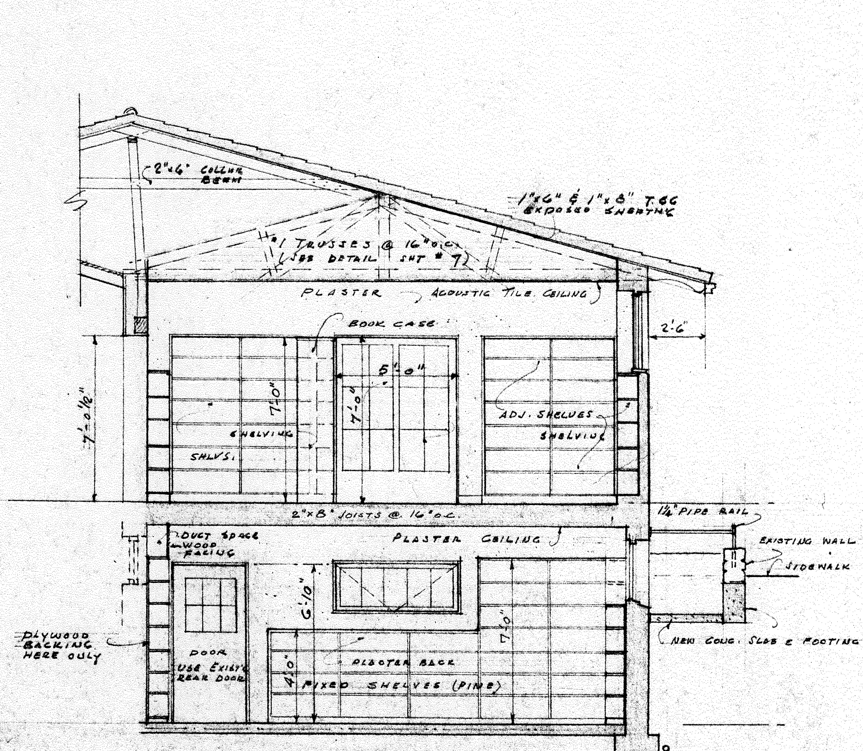
SECTION F-F LOOKING WEST
