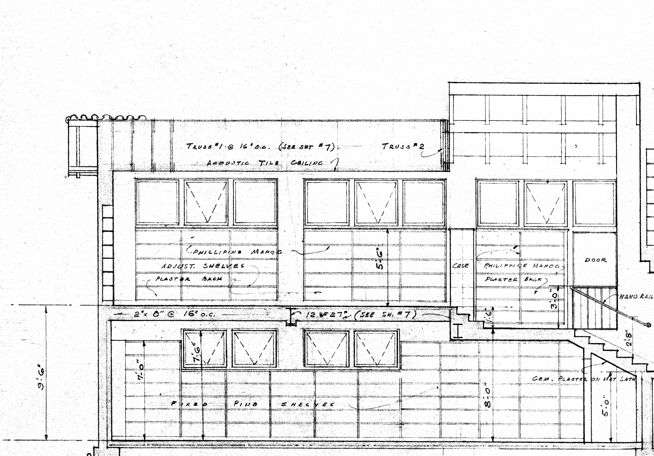
SECTION G-G LOOKING NORTH
