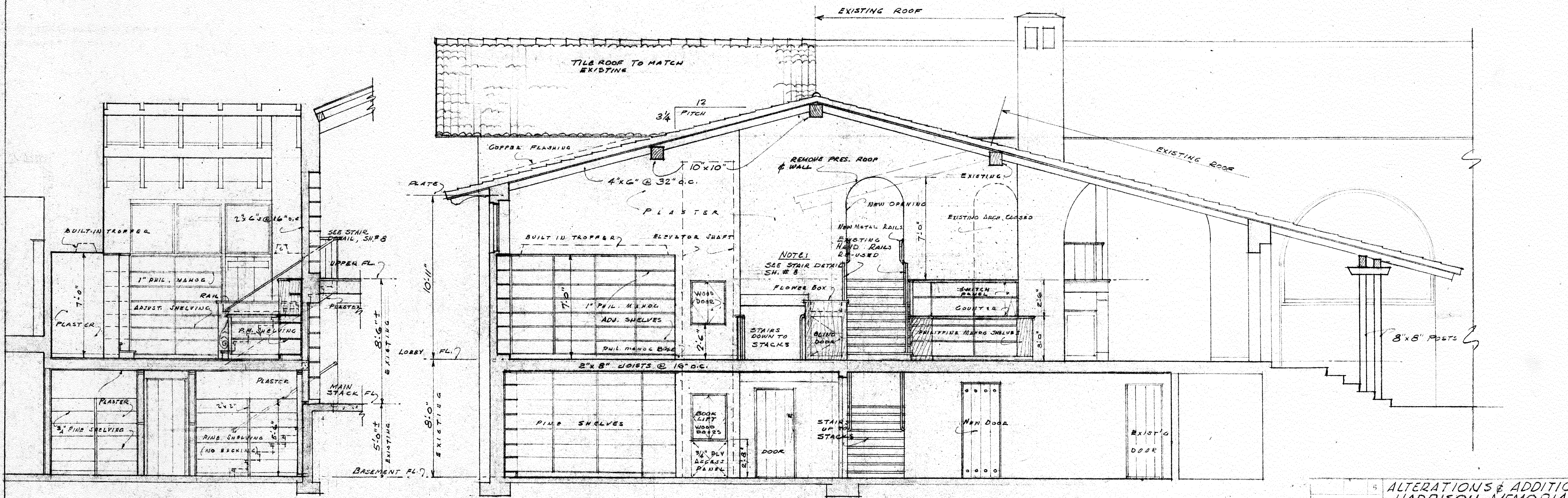
SECTION H-H
