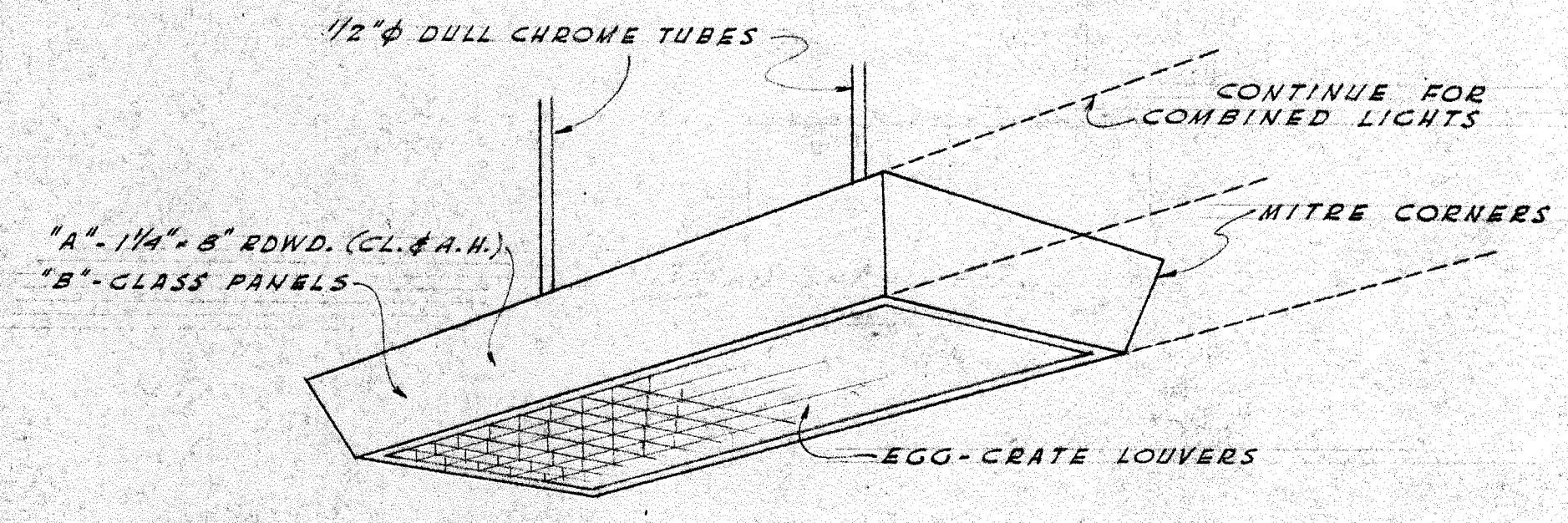
PERSPECTIVE SKETCH OF FIXTURE
