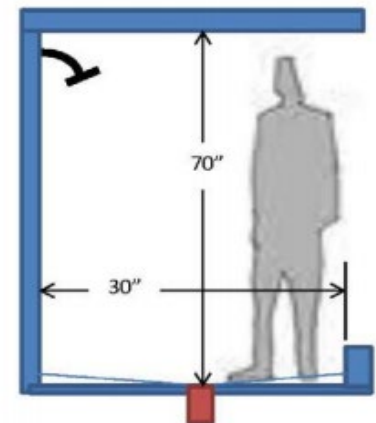
30” diameter must be maintained to a point of not less than 70” above drain
