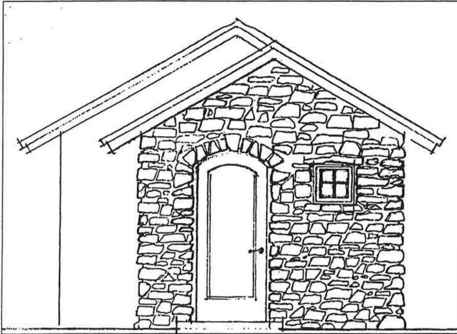
The use of stone on the full exterior of building elements is encouraged. The use of stone only on one elevation, the street facade for example, is discouraged.
